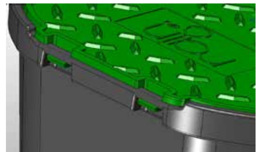
LID CONNECTION
